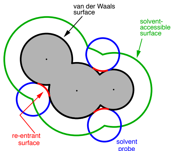
Figure 11.1: Illustration of various solute cavity surface definitions for PCMs. 86 The union of atomic van der Waals spheres (shown in gray) defines the van der Waals (vdW) surface, in black. Note that actual vdW radii from the literature are sometimes scaled in constructing the vdW surface. If a probe sphere (representing the assumed size of a solvent molecule) is rolled over the van der Waals surface, then its center point traces out the solvent accessible surface (SAS), shown in green; the SAS is equivalent to a vdW surface where the atomic radii are increased by the radius of the probe sphere. Finally, one can use the probe sphere to smooth out the sharp crevasses in the vdW surface using the re-entrant surface elements shown in red, resulting in the solvent-excluded surface (SES).
